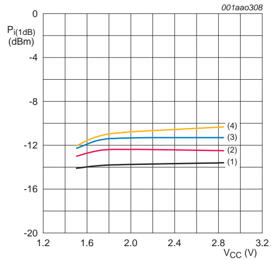
f = 850 MHz. (1) T_{amb} = -40 °C (2) T_{amb} = +25 °C (3) T_{amb} = +85 °C (4) T_{amb} = +125 °C
