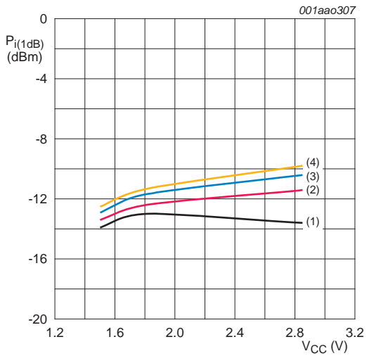
f = 1575 MHz. (1) T_{amb} = -40 °C (2) T_{amb} = +25 °C (3) T_{amb} = +85 °C (4) T_{amb} = +125 °C
