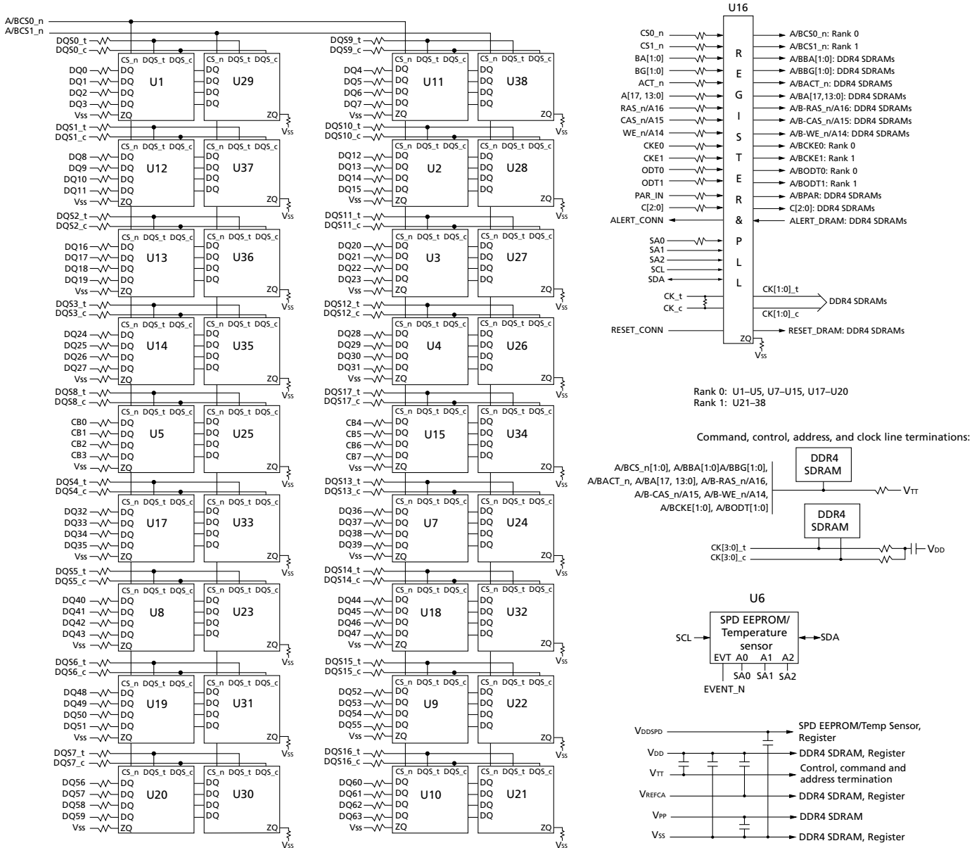
Figure 4: Functional Block Diagram (R/C-B, PCB 1506)
