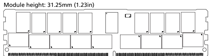
Figure 3: 288-Pin RDIMM (MO-309, R/C-B2)
