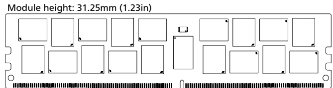
Figure 2: 288-Pin RDIMM (MO-309, R/C-B1)
